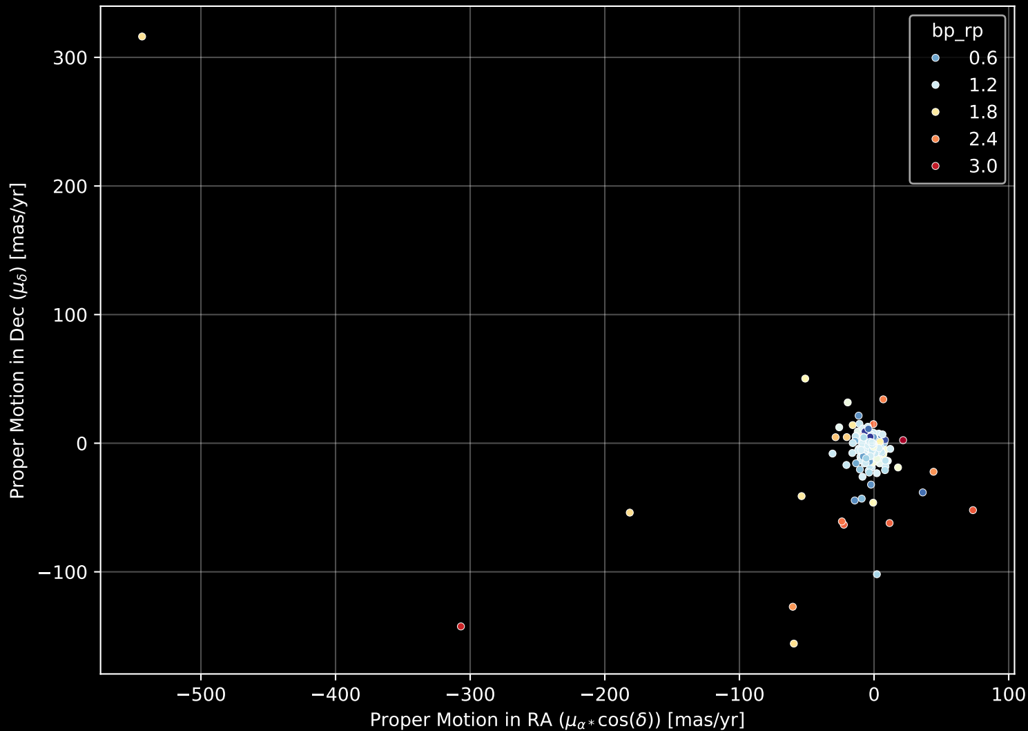
APOGEE DR17 Field: [030+30] Proper Motion Diagram (n= 378)
