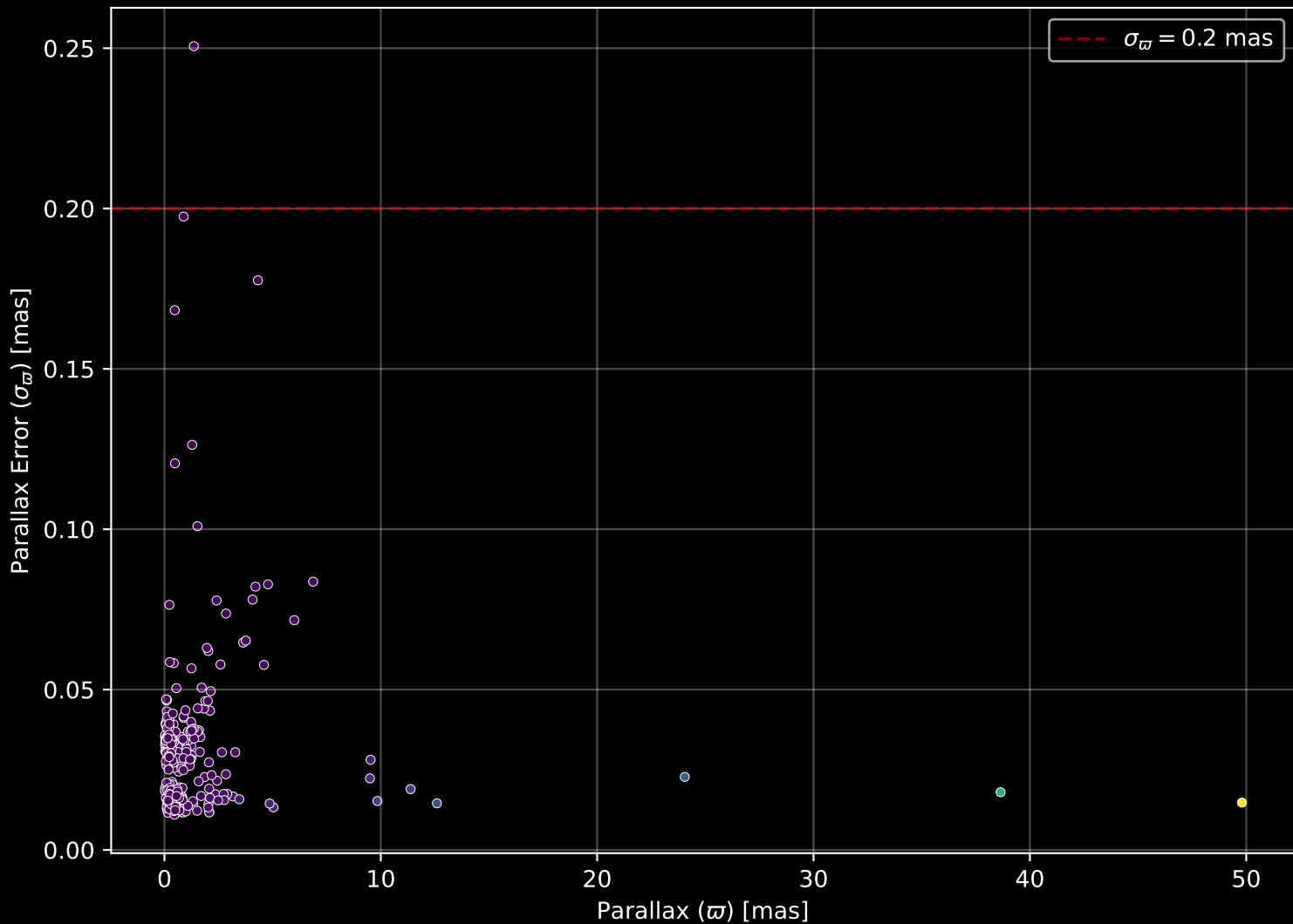
APOGEE DR17 Field: [030+30] Parallax Quality (n= 378)
