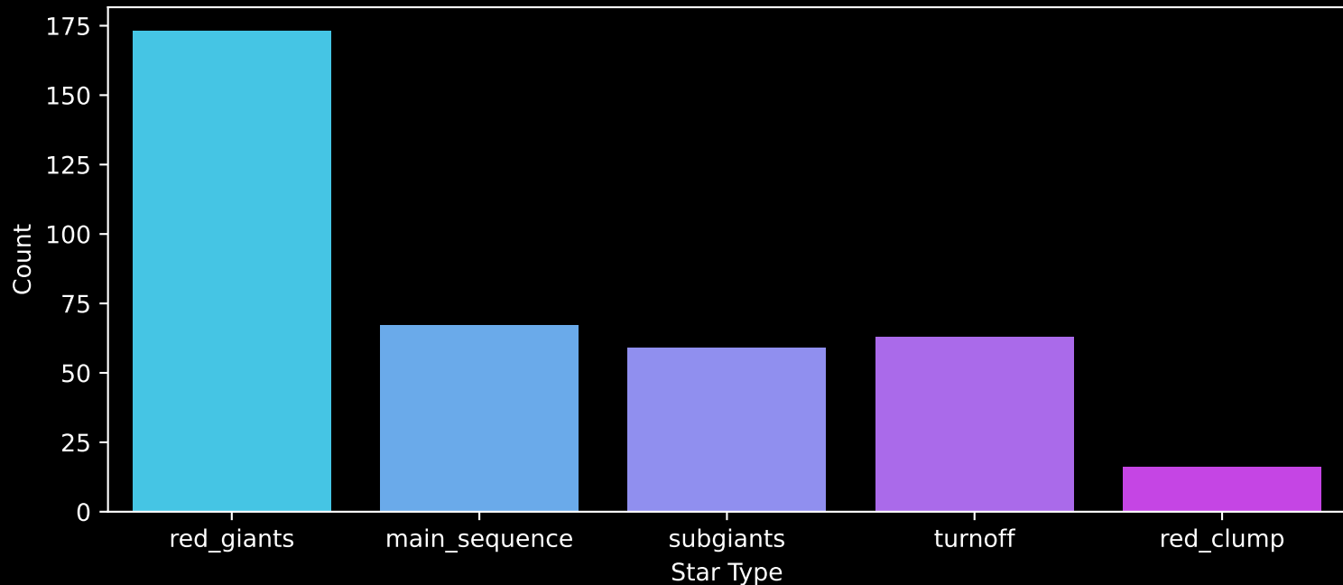
APOGEE DR17 Field: [030+30] Count plot of Star Type
