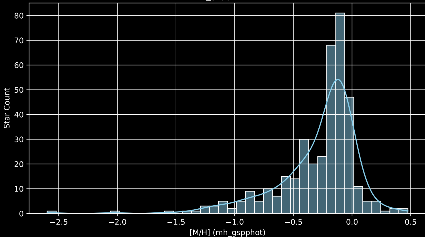
APOGEE DR17 Field: [030+30] [M/H] (mh_gspphot) (n= 378)
