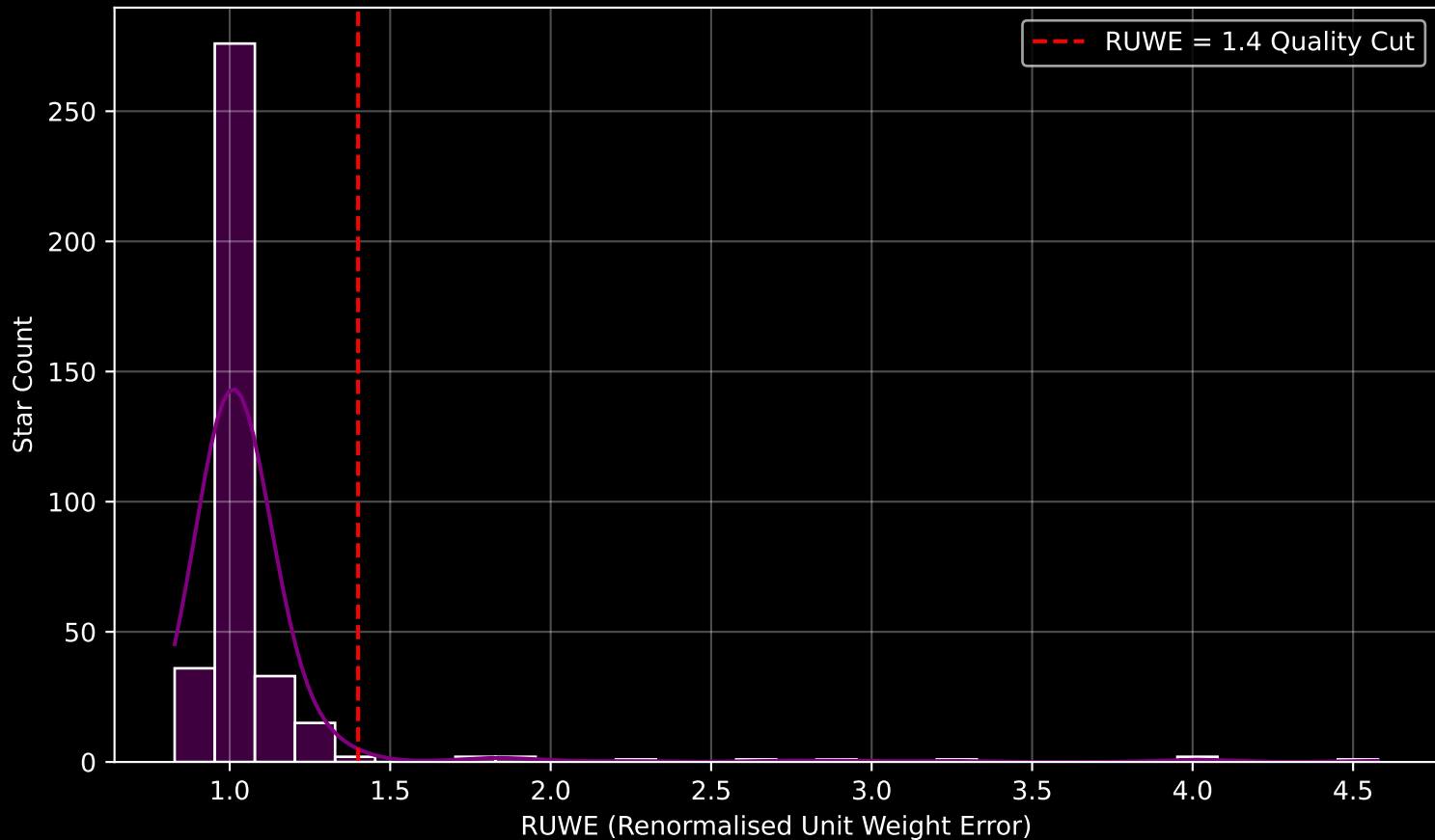
GAPOGEE DR17 Field [030+30] RUWE Distribution (n= 373)
