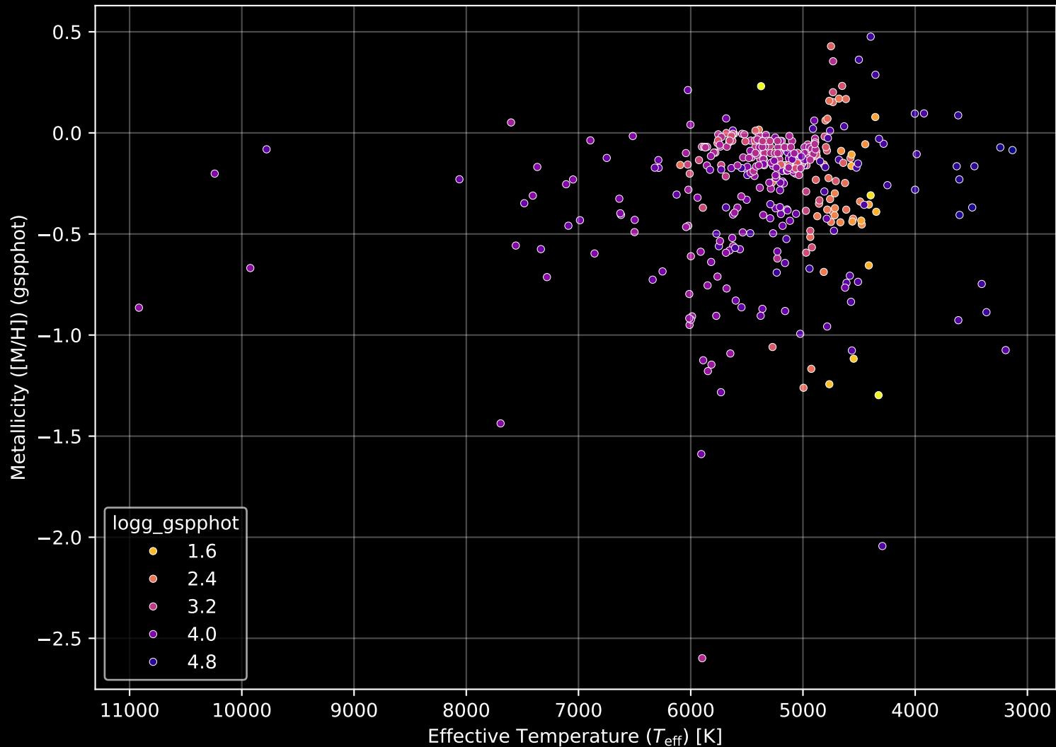
APOGEE DR17 Field: [030+30] Stellar Population Parameters (n= 378)
