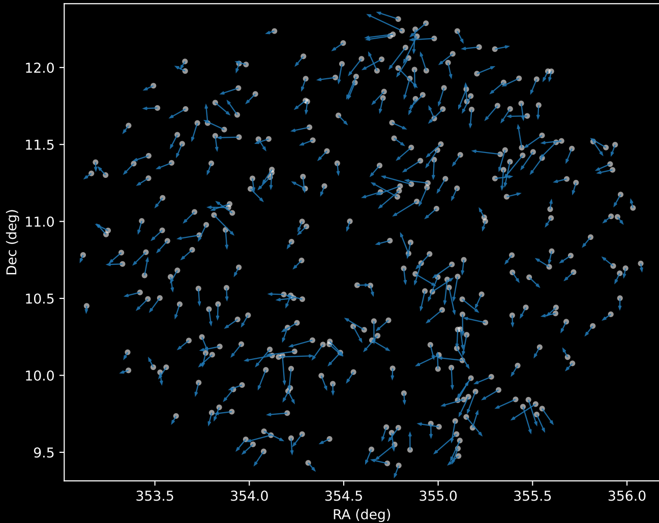
APOGEE DR17 Cluster 0 Proper Motion Vectors (n=328)
