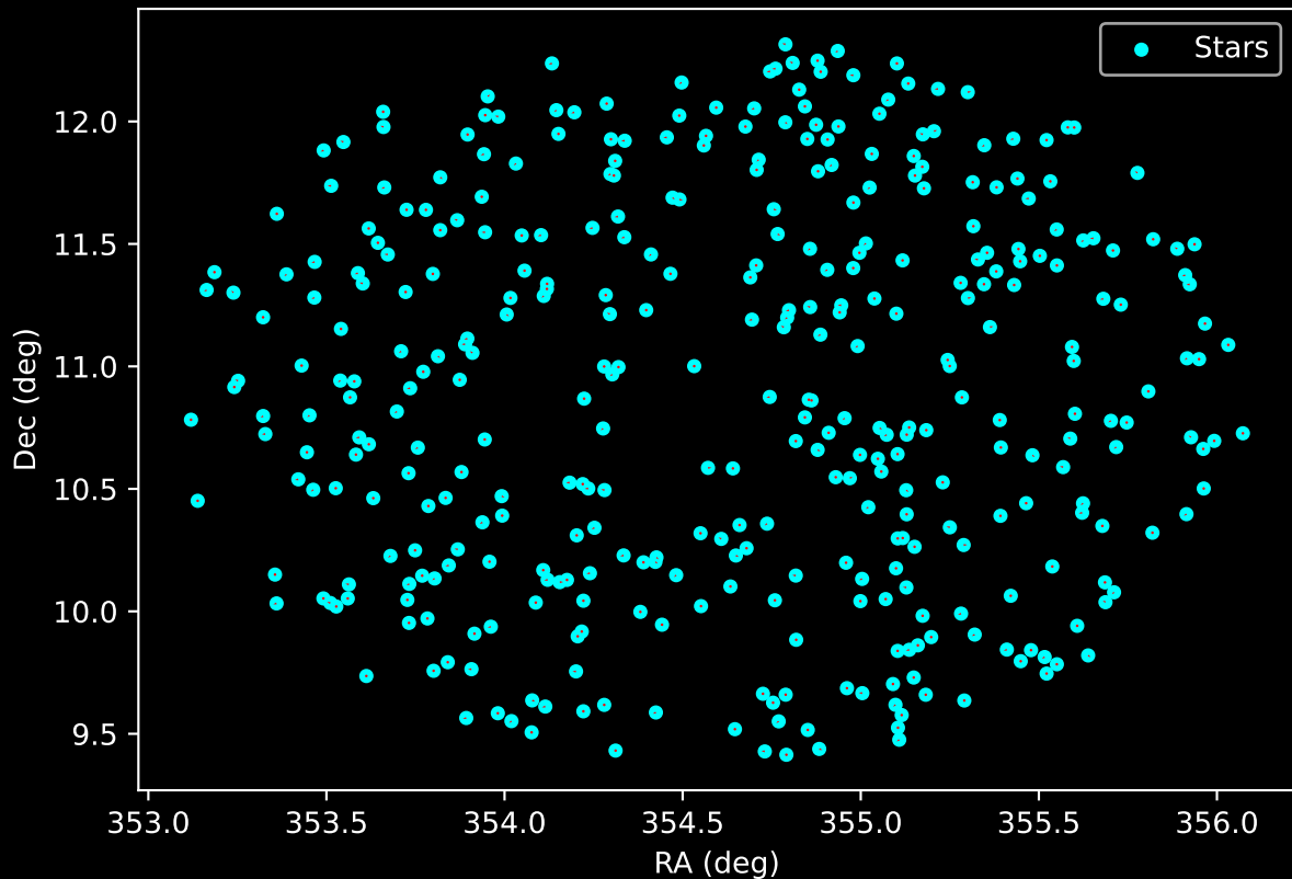
APOGEE DR17 Field: [030+30] Proper Motion Vectors for Gaia Star Field (n= 378)
